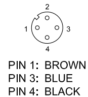
M12 X 1 FEMALE CONNECTOR
