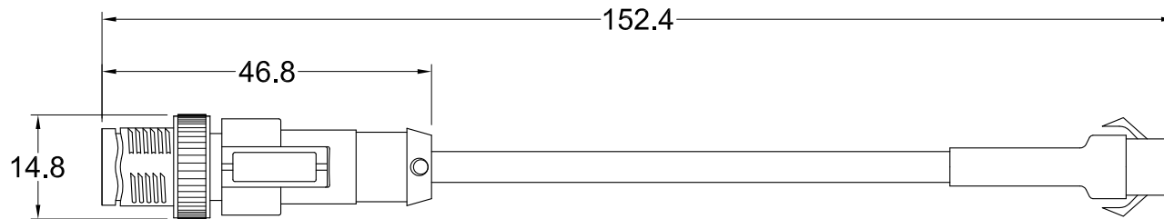
M12 X 1 MALE CONNECTOR
